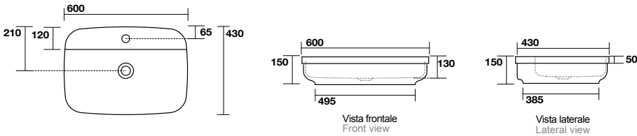
5142 TRIBECA lavabo appoggio o incasso monoforo 60x43 cm. Disponibile anche in KERASAN+TECH. TRIBECA 60x43 cm countertop or semi-recessed basin. Also available in KERASAN+TECH.
