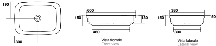
5143 TRIBECA lavabo appoggio o incasso 60x38 cm. Disponibile anche in KERASAN+TECH. TRIBECA 60x38 cm countertop or semi-recessed basin. Also available in KERASAN+TECH.
