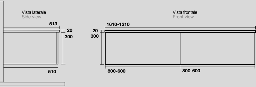
7441 Mobile sospeso cm 120 con 2 cassetti push&pull 120 cm wall-hung vanity unit with 2 push to open drawers
