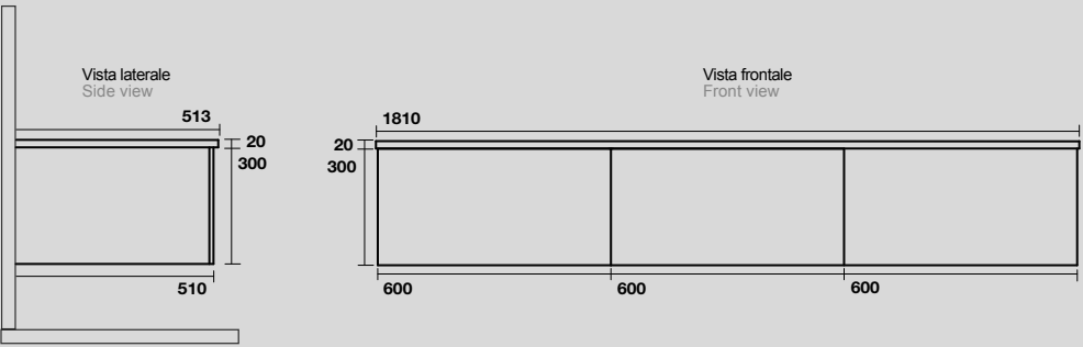
7443 Mobile sospeso cm 180 con 3 cassetti push&pull 180 cm wall-hung vanity unit with 3 push to open drawers
