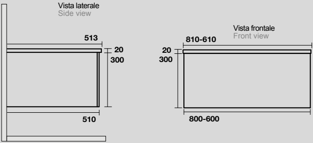
7439 Mobile sospeso cm 60 con cassetto push&pull 60 cm wall-hung vanity unit with push to open drawer
