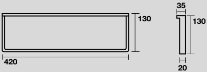
9209 Piede in metallo per mobili Metal support for vanity units
